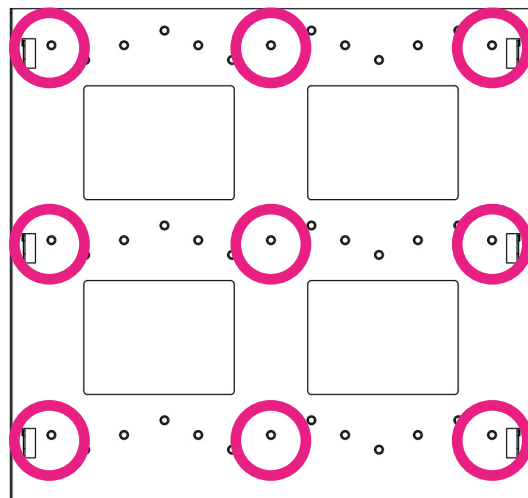
ChargeLite Wall Bracket showing 9 fixing points
